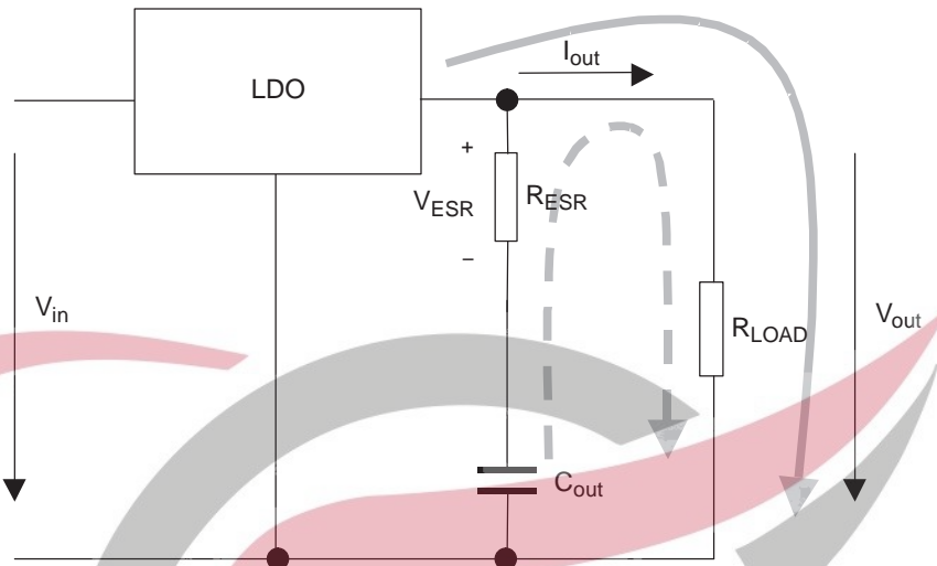
Figure 48. LDO Output Stage with Parasitic Resistances ESR
